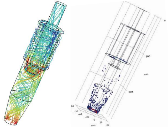
Cyclonic Separation
