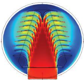
Schoepentoeter Inlet Device
